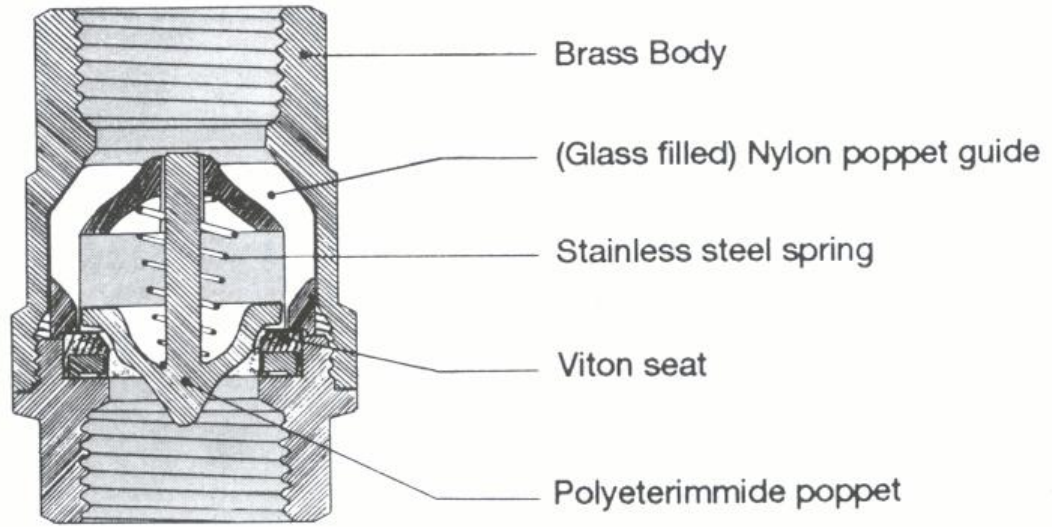
OIL CHECK VALVE CUTAWAY VIEW
